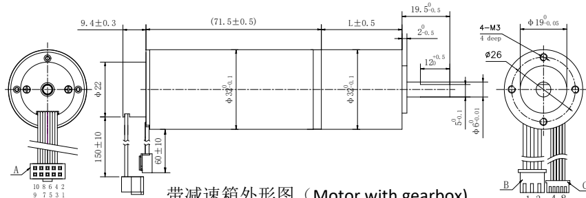
带减速箱外形图 (Motor with gearbox)
