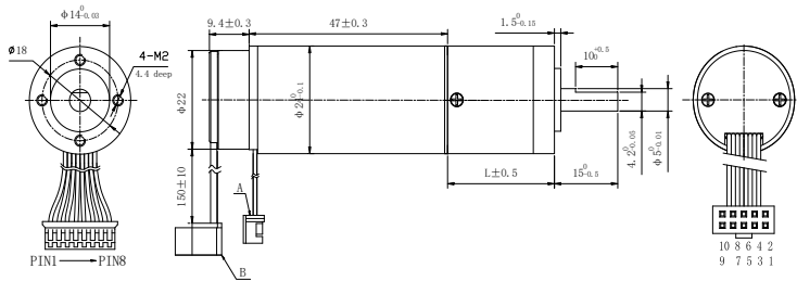
带减速箱外形图 (Motor with gearbox)
