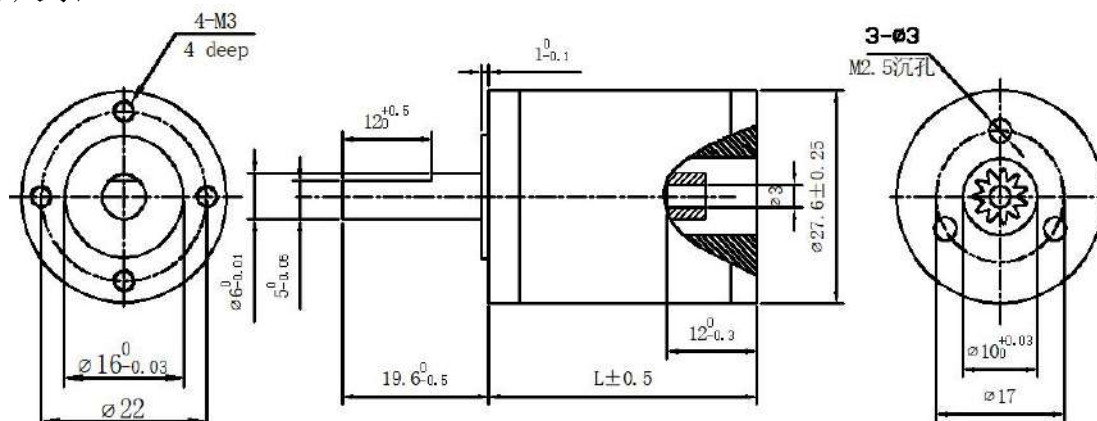
标准减速比型式/Gearboxes Specifications
